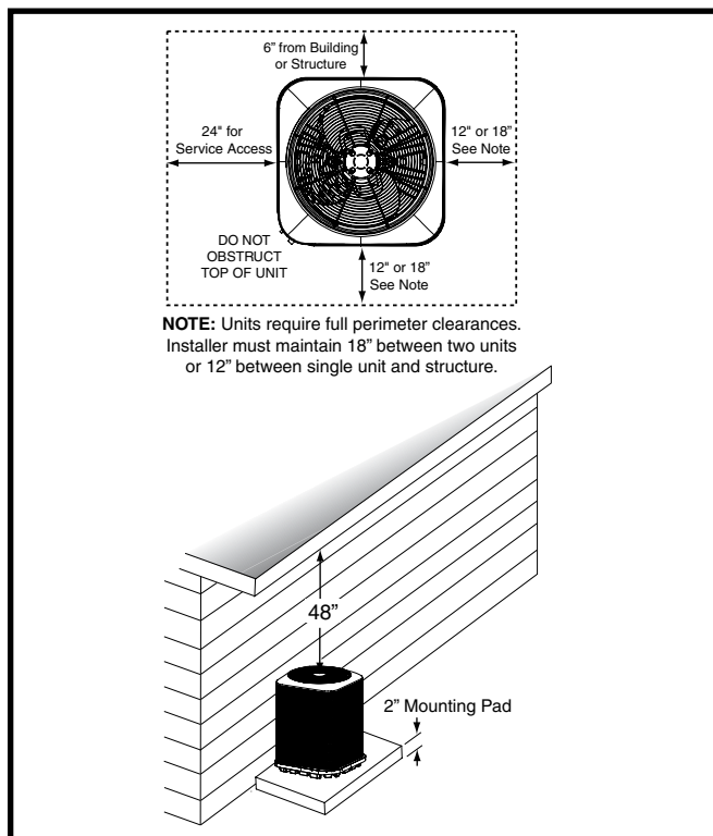
Figure 1. Clearance Requirements
