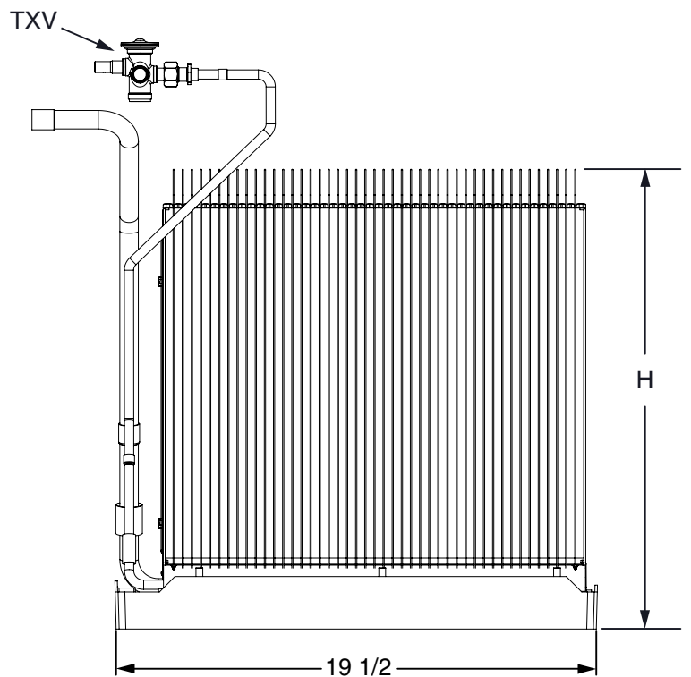
Figure 6. C7 Coil Dimensions (with TXV)
