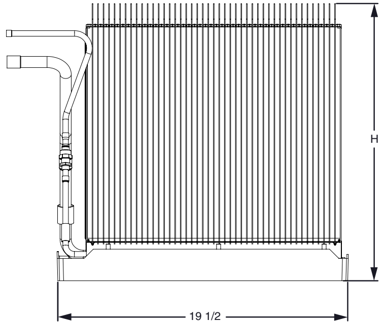
Figure 5. C7 Coil Dimensions (without TXV)
