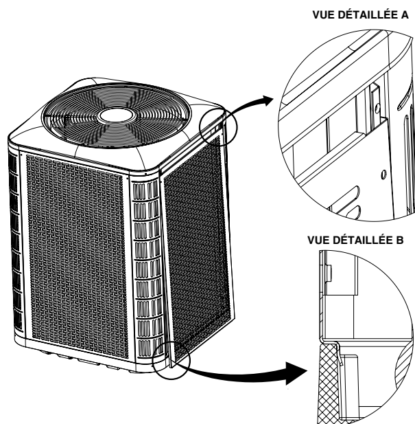
Figure 4. Installation du panneau
