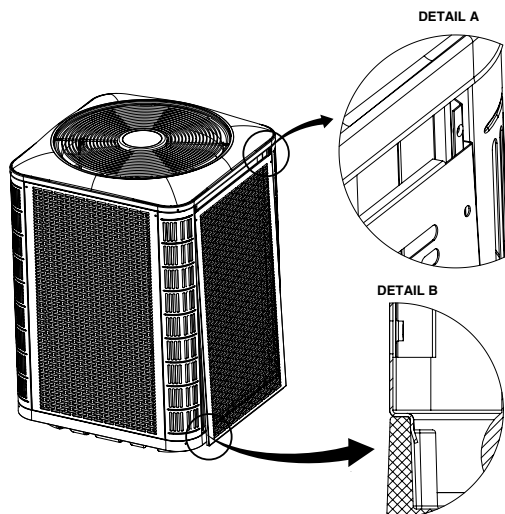
Figure 4. Installation du panneau
