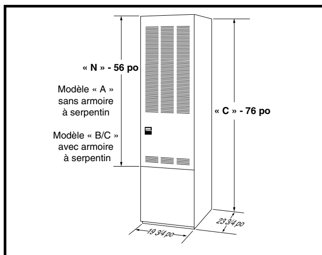
Figure 4. Dimensions totales
