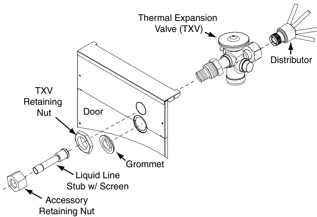
Figure 6. TXV Assembly
