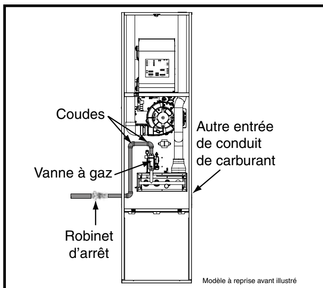
Figure 18. Raccordements de gaz typiques
