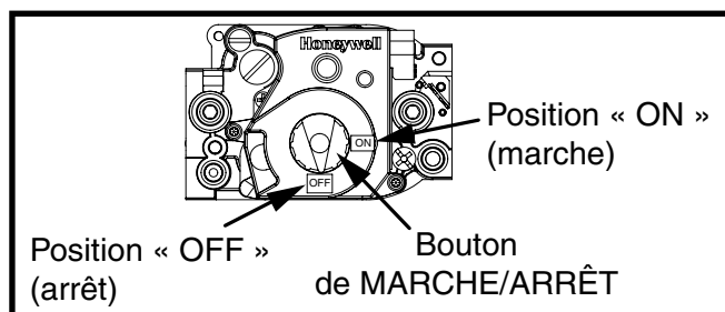
Figure 3. Robinet de gaz Honeywell
