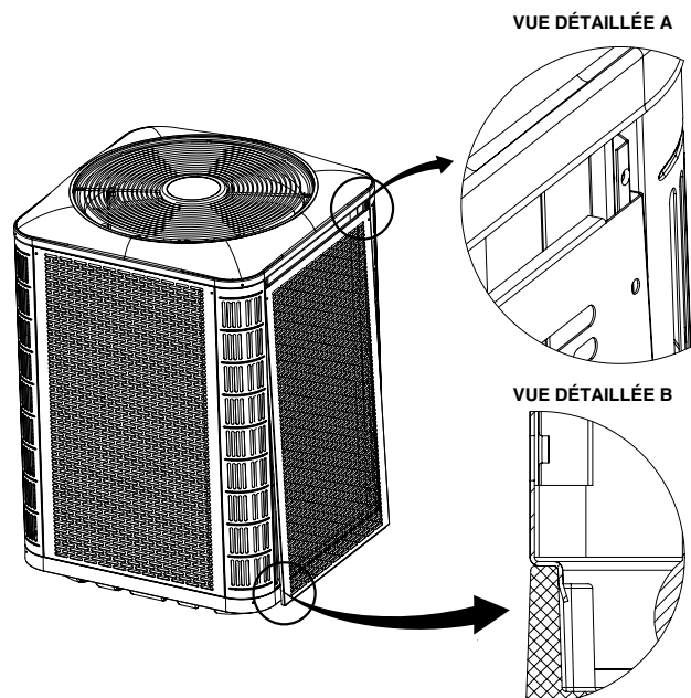
Figure 5. Installation du panneau
