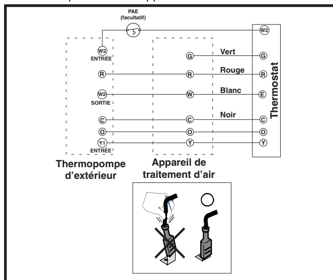
Figure 2. Raccordements de thermostat typiques
