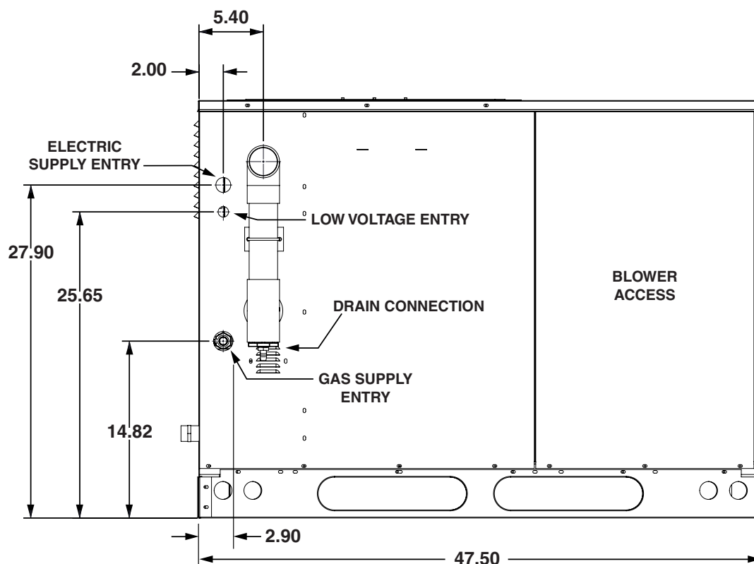
Side View
