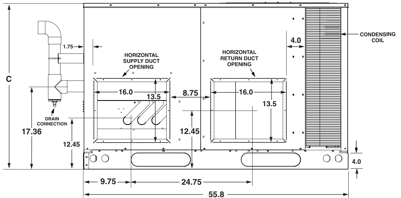
Back View
