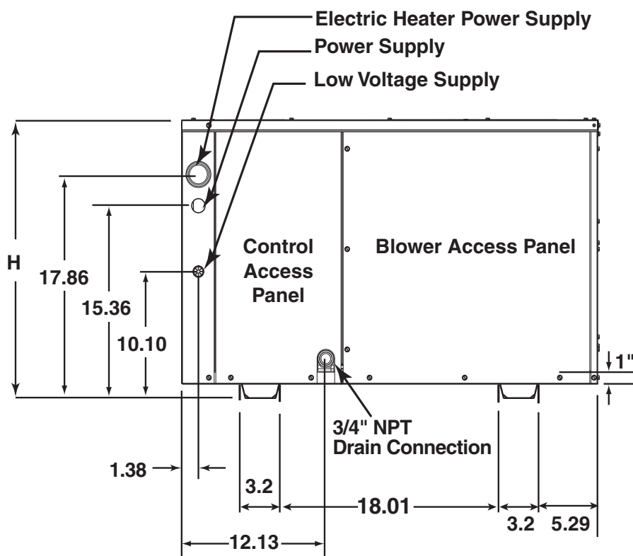
Side View
