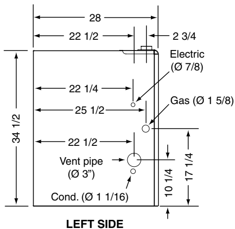
FG7SL 90+ High Efficiency Downflow Series
