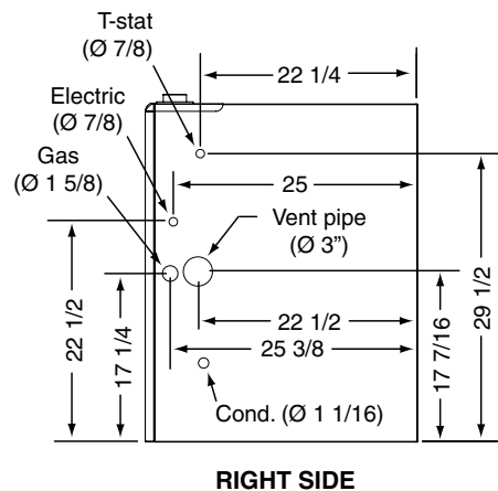
FG7SL 90+ High Efficiency Downflow Series
