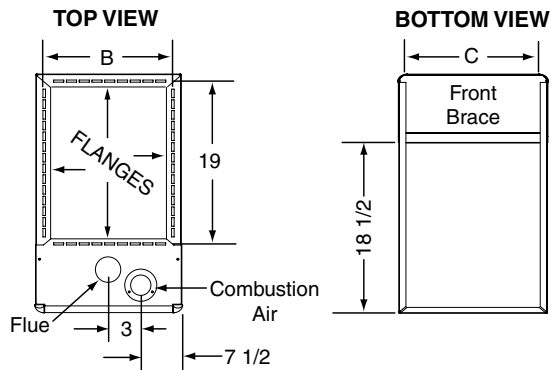
FG7SC 90+ High Efficiency Upflow/Horizontal Series
