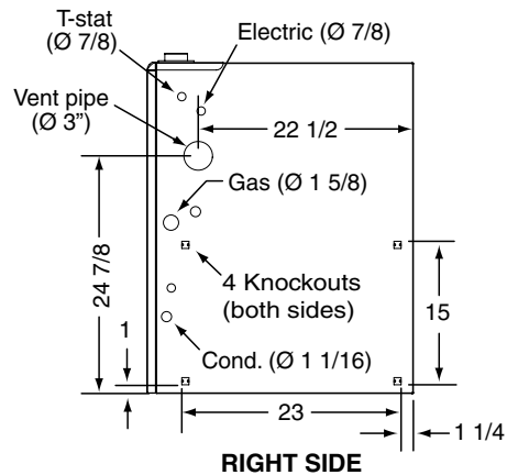
FG7SC 90+ High Efficiency Upflow/Horizontal Series
