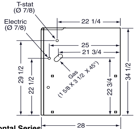
FG7TA 80+ High Efficiency Upflow/Horizontal Series
