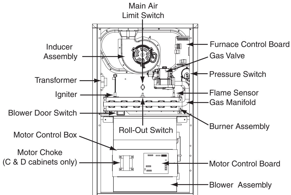
Upflow/Horizontal Gas Furnace Components
