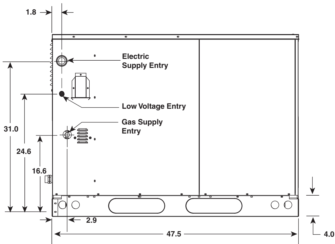
Side View
