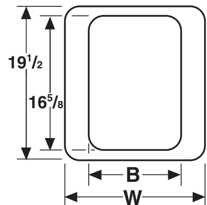
Figure 4. Drain Pan Dimensions
