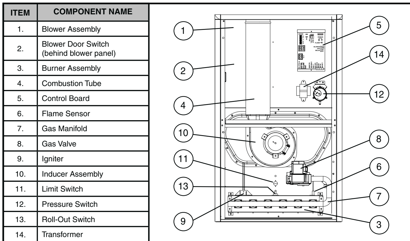
Downflow Gas Furnace
