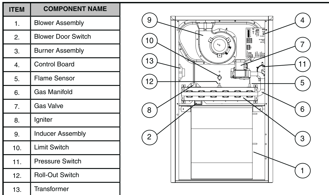
Upflow/Horizontal Gas Furnace
