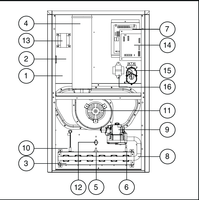
Downflow Gas Furnace
