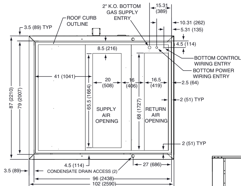
BOTTOM VIEW
