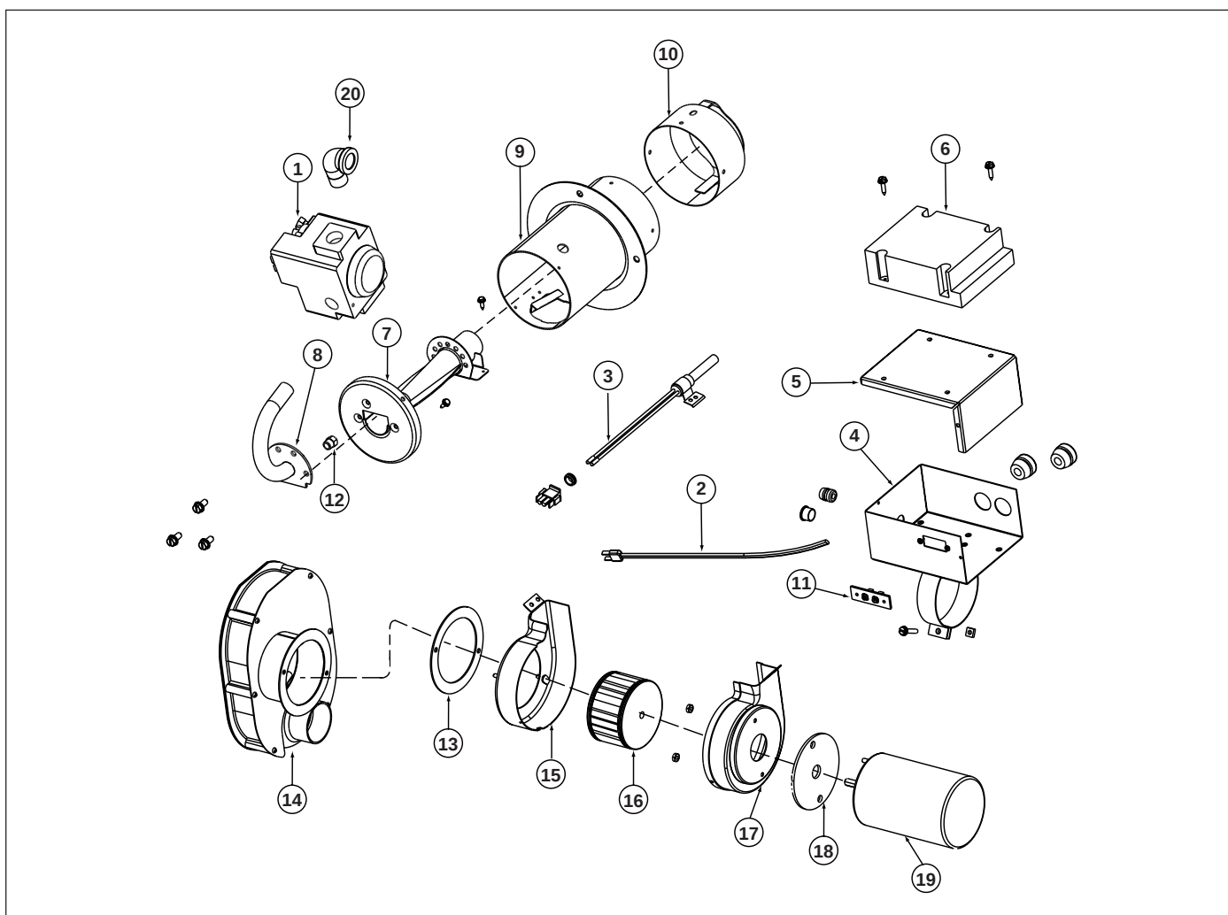
Figure 3. Gas Burner Diagram
