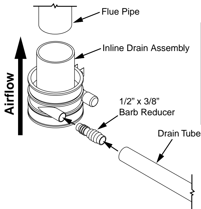
Figure 1. Inline Drain Assembly Diagram
