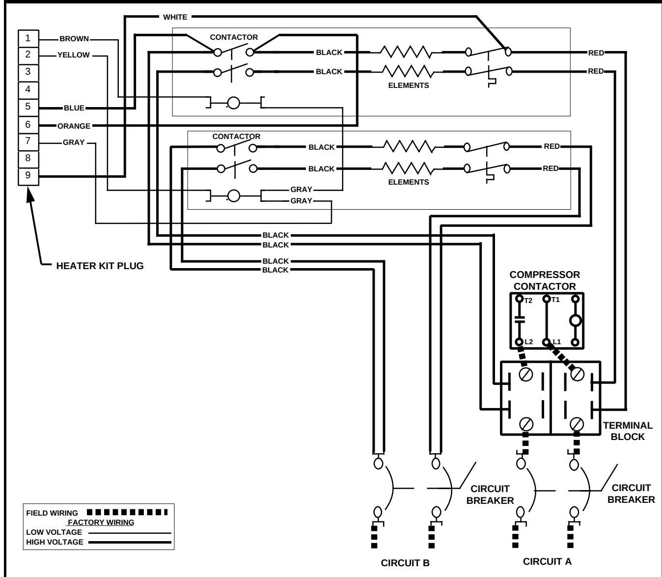
Wiring Diagram #6 - Single Phase - 20 KW, 2 Circuit
