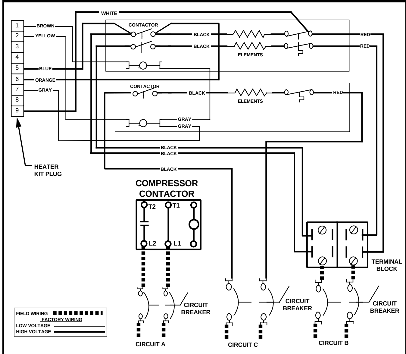
Wiring Diagram #5 - Single Phase - 15 KW, 3 Circuit
