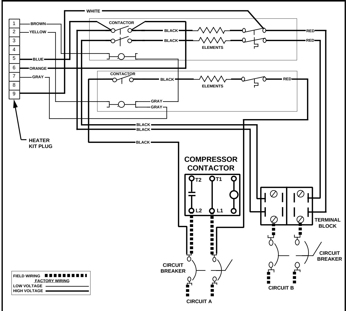
Wiring Diagram #4 - Single Phase - 15 KW, 2 Circuit (Heat Pump Application)
