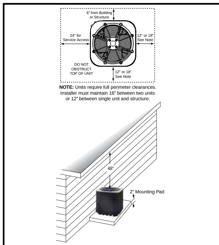
Figure 1. Clearance Requirements
