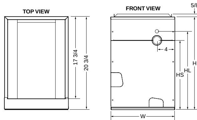
Figure 5. Coil Dimensions
