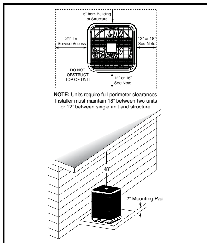
Figure 1. Clearance Requirements
