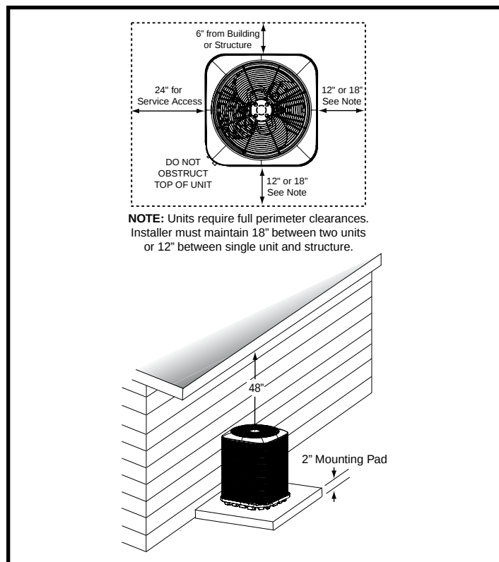
Figure 1. Clearance Requirements
