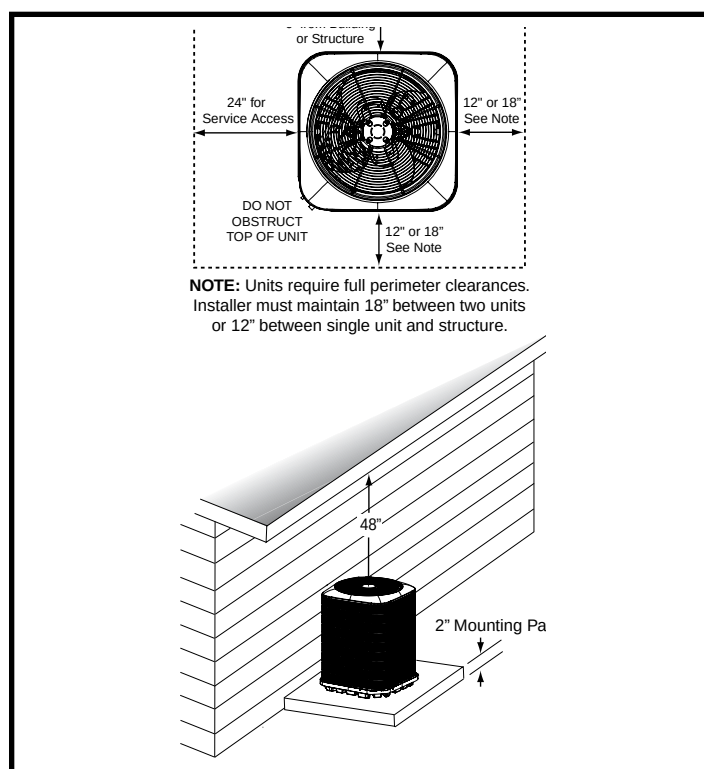
Figure 1. Clearance Requirements
