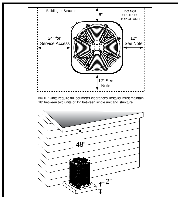
Figure 1. Clearance Requirements
