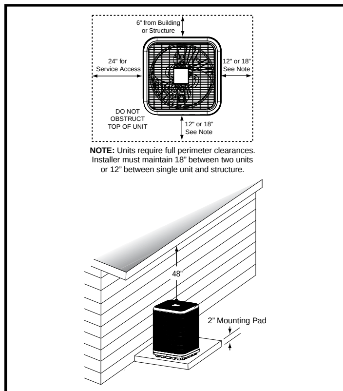
Figure 1. Clearance Requirements
