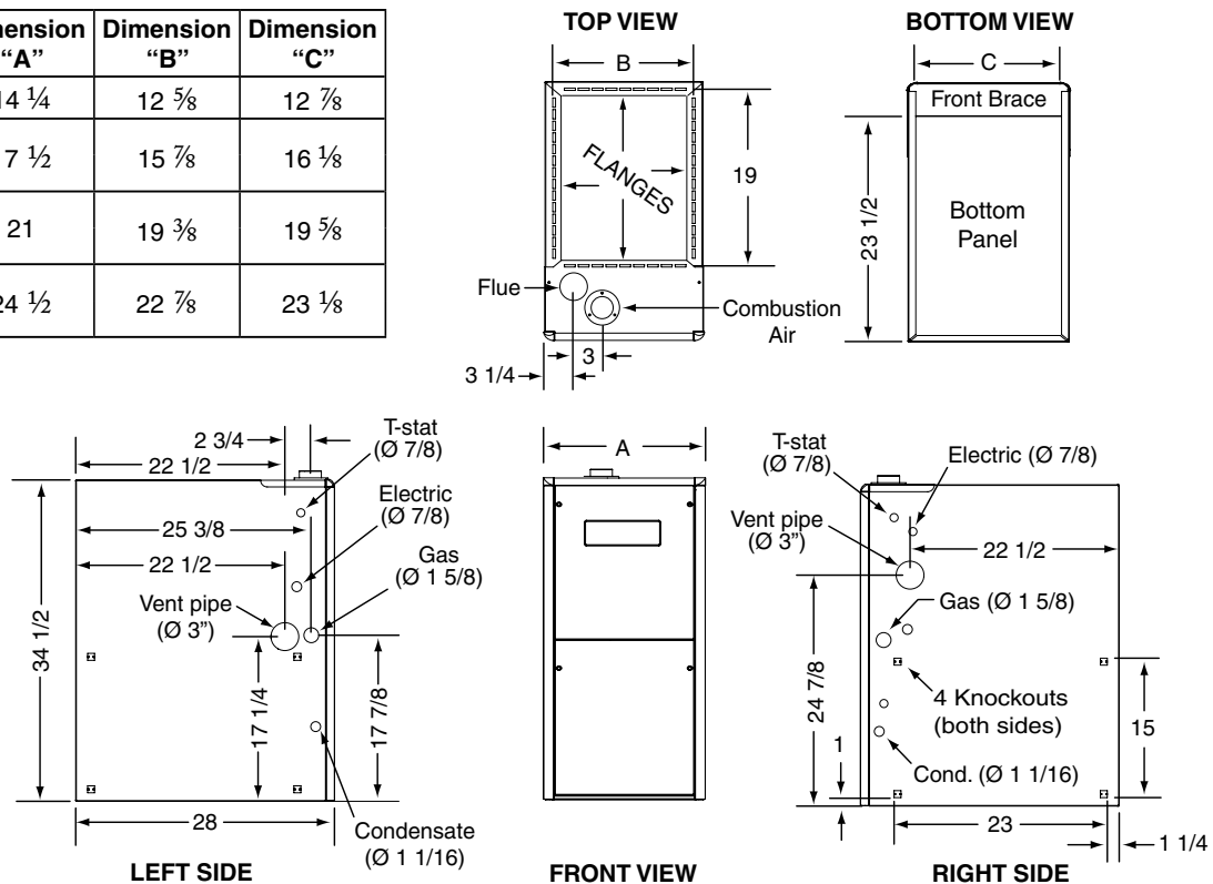
KG7SC 90+ High Efficiency Upflow/Horizontal Series
