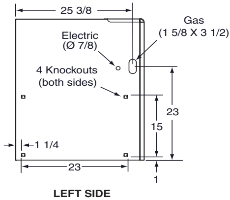
MGC2SA 80+ High Efficiency Upflow/Horizontal Series
