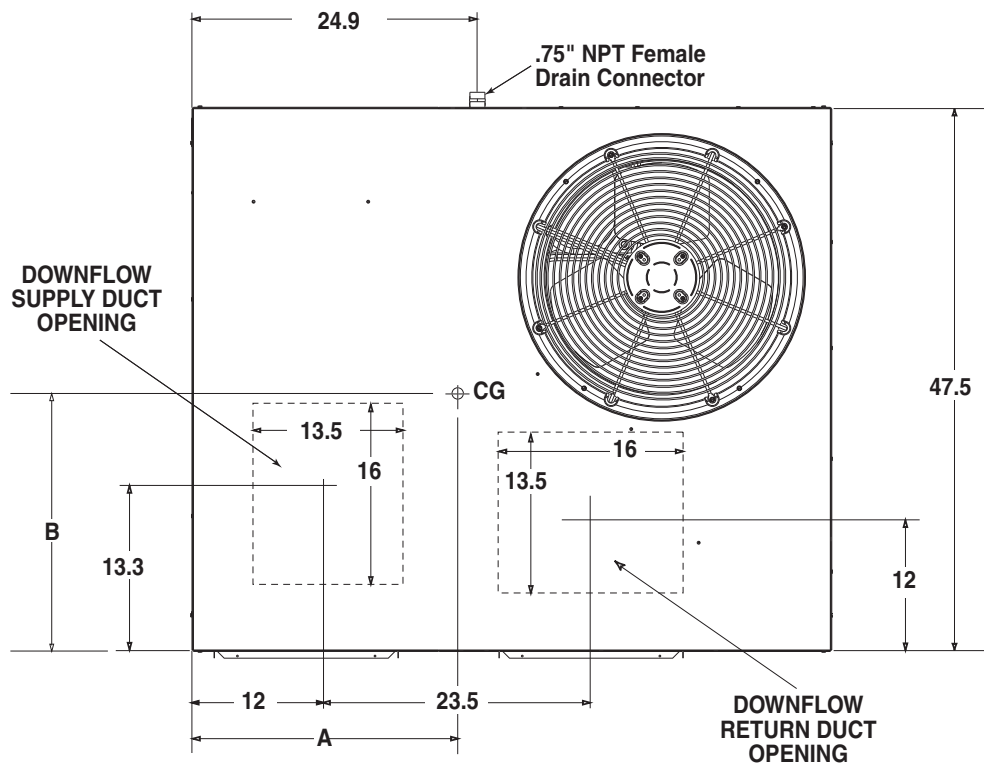
Top View
