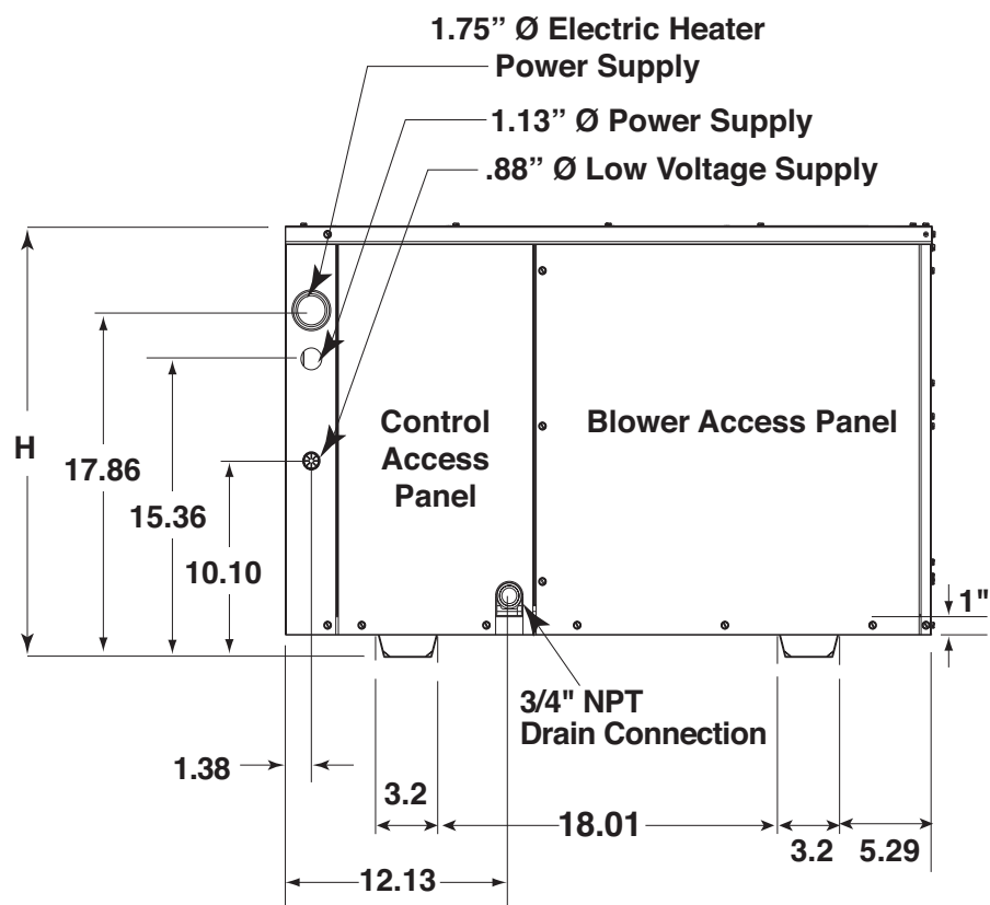
Side View
