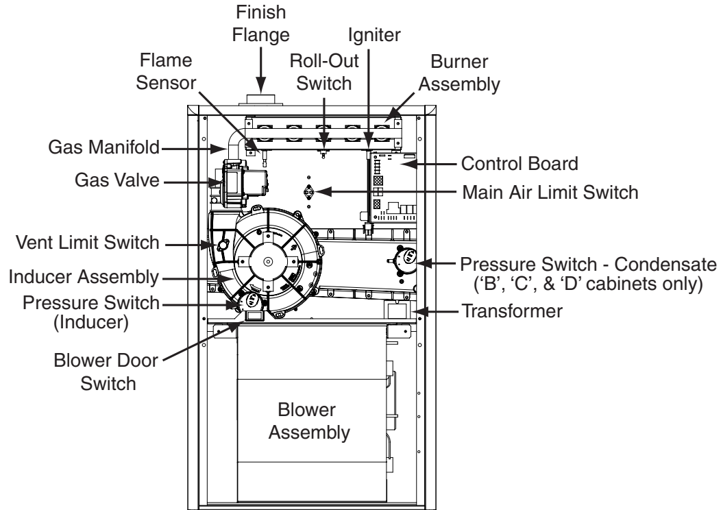
Upflow/Horizontal Gas Furnace Components
