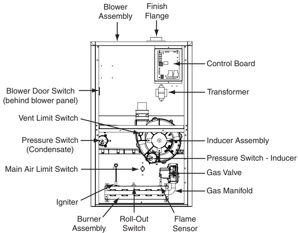
Downflow Gas Furnace Components
