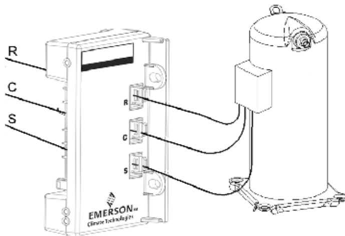
Figure 1 Wires Pulled Through Module
