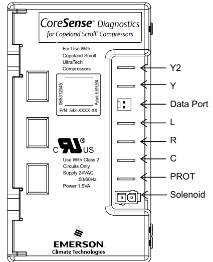
Figure 2 Terminal Locations
