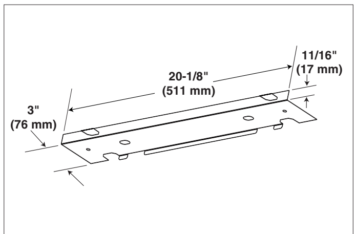
Figure 3. Optional Rear Mounting Plate (P/N 389080)
