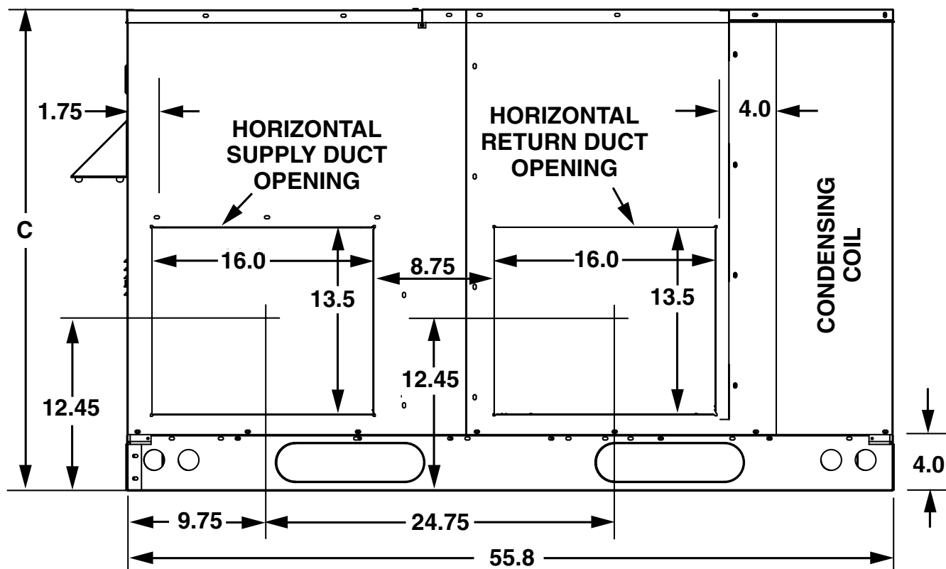
Back View
