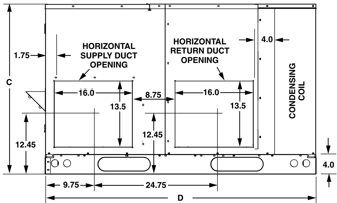
Back View
