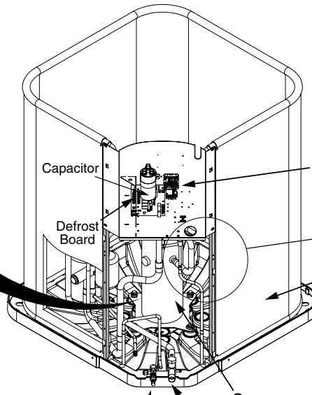
Compressor
