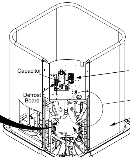
Compressor
