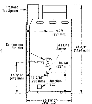
Right Side
