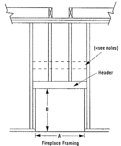
Fireplace Framing
