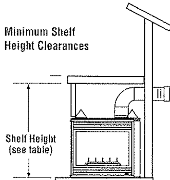
Shelf Above Fireplace With Top Venting
