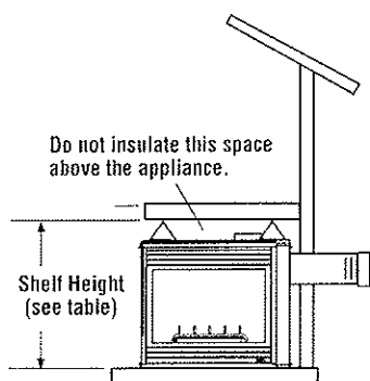
Shelf Above Fireplace With Side Venting
